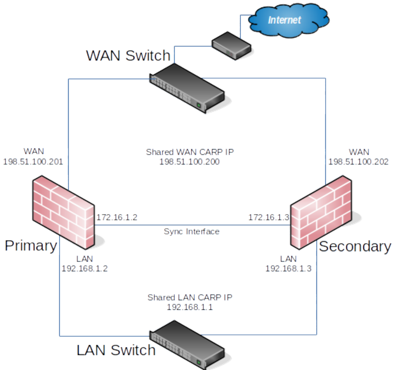
Fig. 1: Example HA Network Diagram
