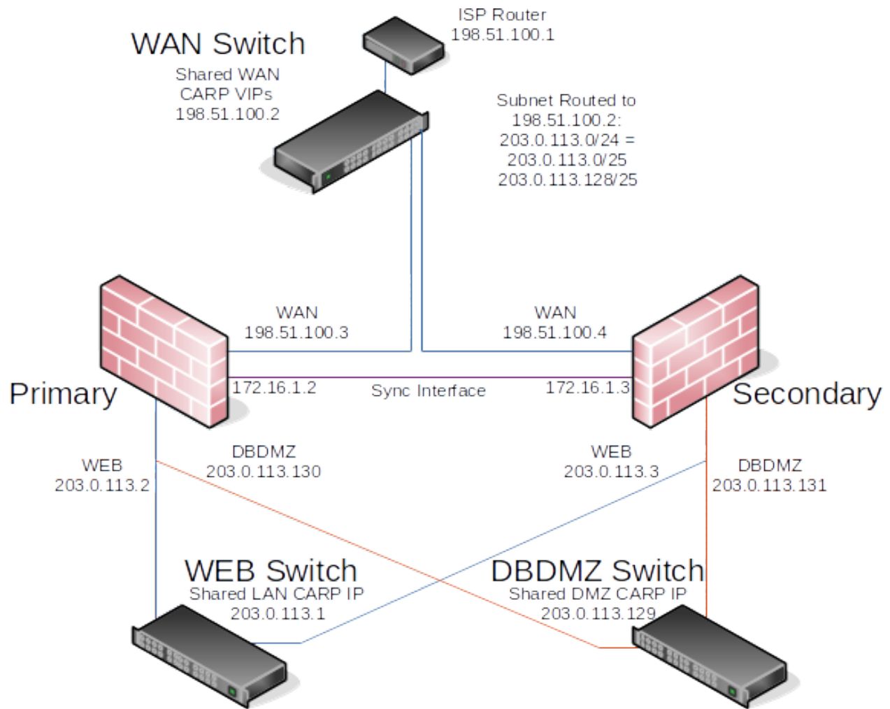
Fig. 7: Diagram of HA with Routed IPs
