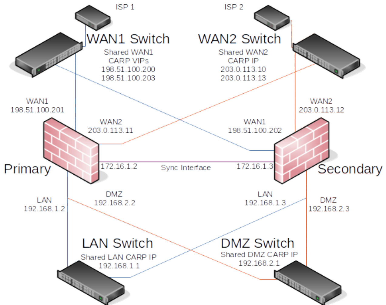
Fig. 5: Diagram of Multi-WAN HA with DMZ
