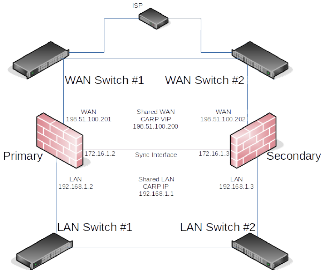
Fig. 8: Diagram of HA with Redundant Switches
