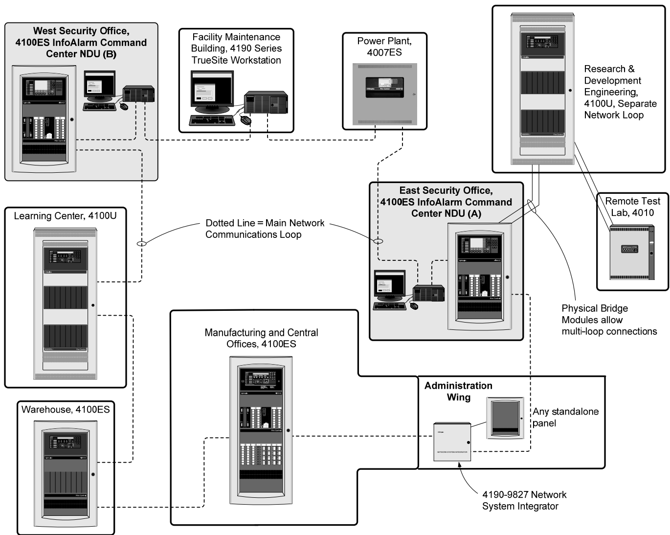
Figure 2. Multiple Building Network Application
