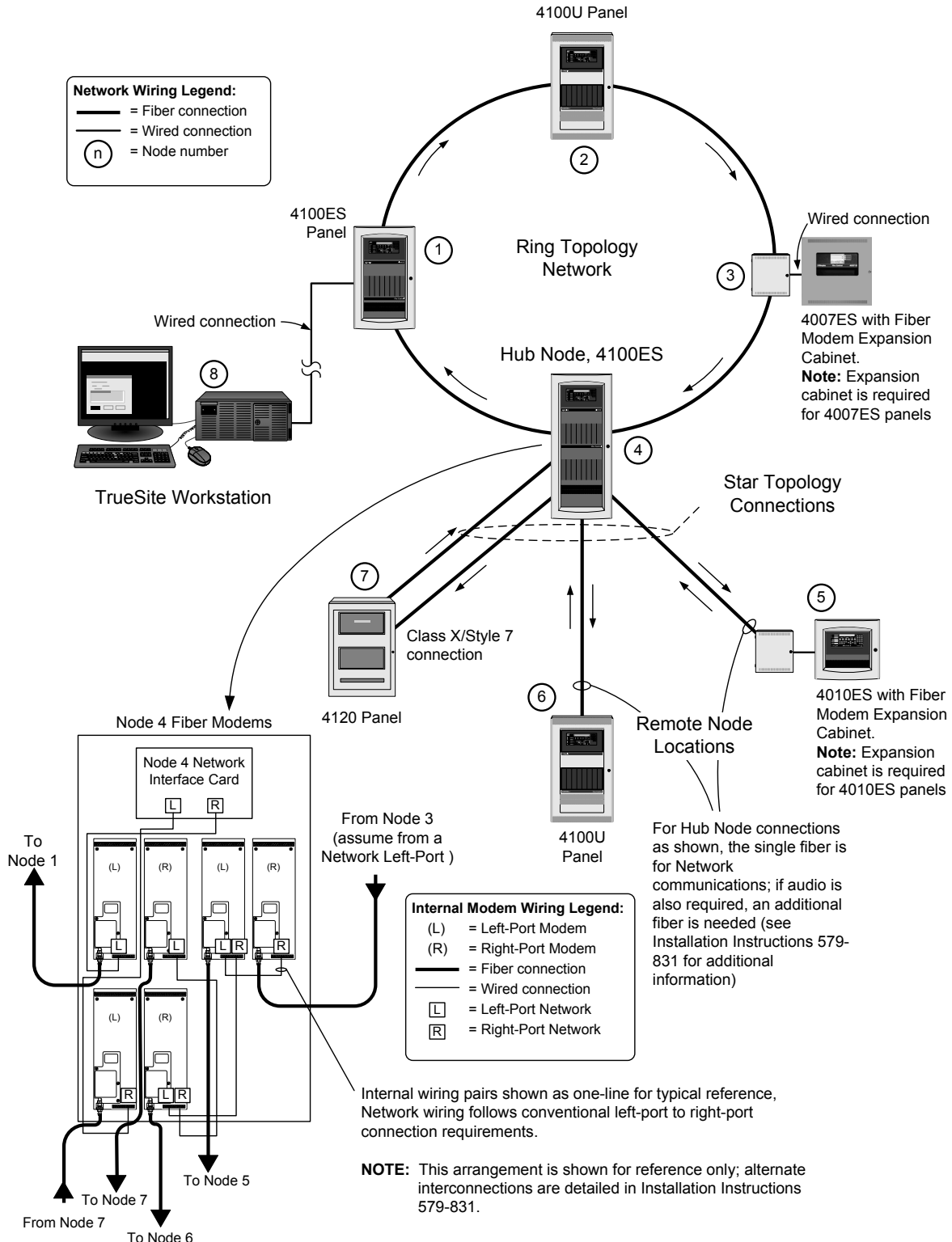
Figure 3. Network Connections using Multiple Communication Signal Fiber Modems
