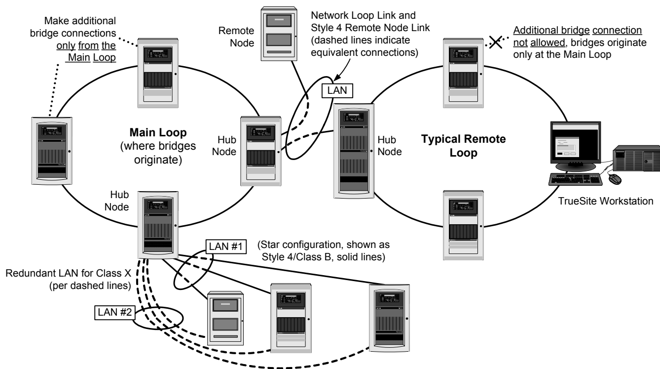
Figure 5. Multiple Loop Network with TCP/IP Modems
